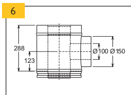
Sopouch 100/150 (bez spony)
