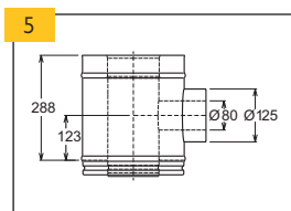
Sopouch 80/125 (bez spony)
