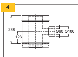
Sopouch 60/100 (bez spony)
